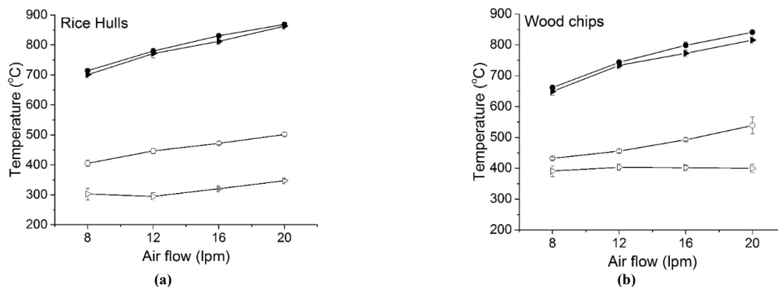
Figure 2. Airflow rate and insulation effects on combustion zone temperature and average temperature of TLUD gasification of (a) rice hulls and (b) wood chips: \blacktriangle = without insulation, \bullet = with insulation, \triangle = average temperature without insulation, \circ = average temperature with insulation.
