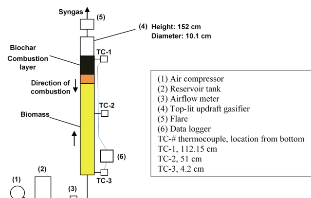
Figure 1. Schematic diagram of top-lit updraft gasifier.
